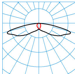
LIQ 50N-SB3L-LRA/1200-727 2G1 ETDD (CLO end value) TX277992
