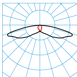
LIQ 50N-SB3L-LRA/1200-727 2G1 ETDD (CLO initial value) TX277821
