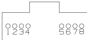
8F MPO FERRULE POSITION CONNECTOR END VIEW (KEY UP)
