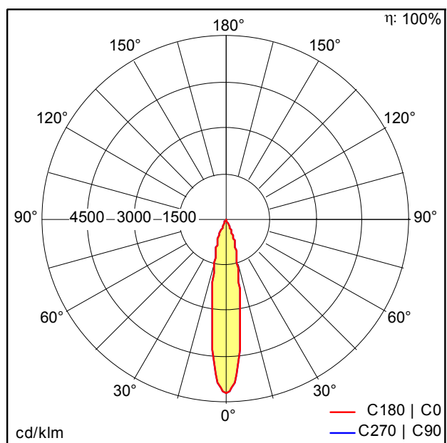
STx1071.ltd
