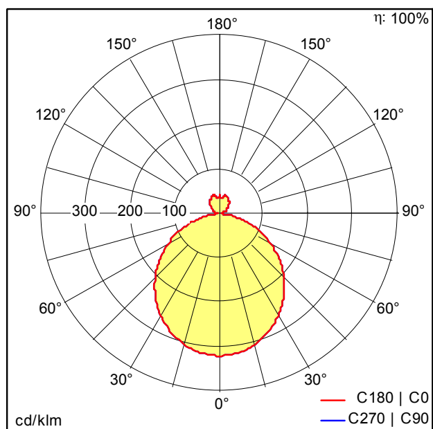
ZS_Lanos_500mm_OP_5000lm.Idt
