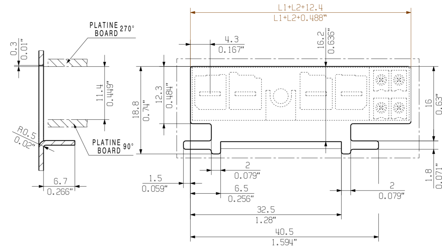
MIN. FRONT PLATE CUT-OUT
