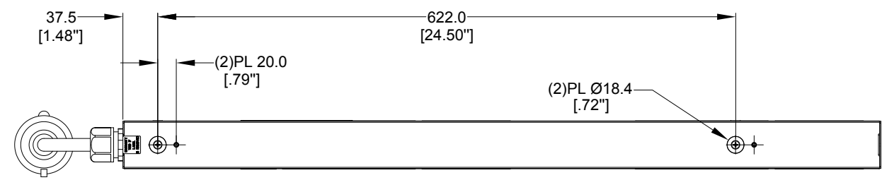
REAR VIEW
