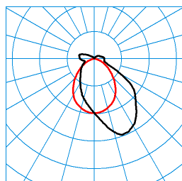
TugraHE Act 12 PAW 50-840 ETDD8 01 (ACTDCW) TX302549 ■ C0 - C180 ■ C90 - C270 DIN 5040: B40 UTE: 0,87 E + 0,13 T CEN Flux Code: 48 79 93 87 100 7 25 60 13
