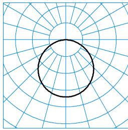
Skeo Circ MultiLC WD2 1G1Y ETDD E3 (nw) ■ C0 - C180 TX278670 UGR I = 24,0 UGR q = 24,0 DIN 5040: A40 UTE: 1,00 E CEN Flux Code: 46 78 96 100 100
