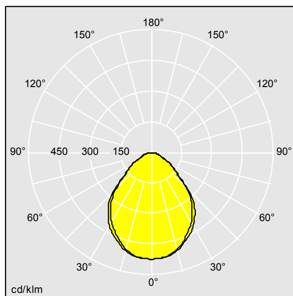
D44261AA_EQL_840_HF_L1000_LRO_SR_.ldt
