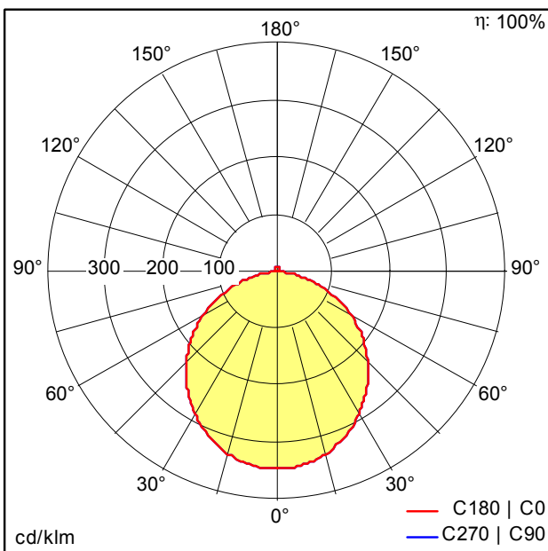
D36853AA_ONDA2_A_D590_LED5800-840.ltd
