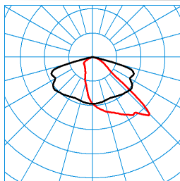
Cuvia 60-AB6L-LR/7500-740 12G1S TX054514 ■ C0 - C180 ■ C90 - C270 DIN 5040: A30 UTE: 1,00 E CEN Flux Code: 40 75 98 100 100
