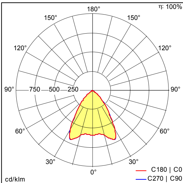
D43023_MIRL_NIV_3800-830_M600L_NB_EVG_WH.Idt
