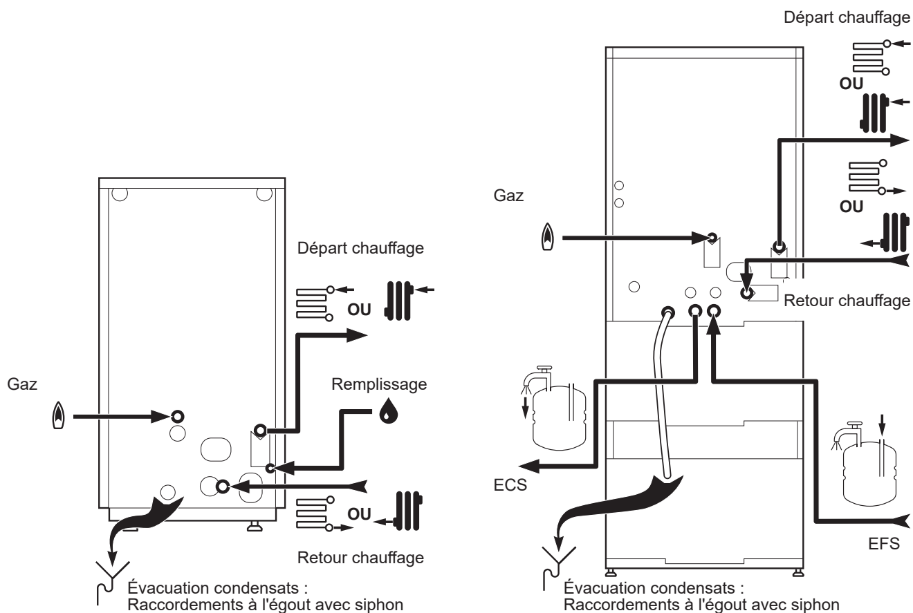
fig. 16 - Raccordements hydrauliques
