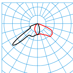
LIQ 50N-FL1L/4200-740 4G1 ET (CLO initial value) TX278320 ■ C0 - C180 ■ C90 - C270 DIN 5040: A40 UTE: 1,00 F CEN Flux Code: 43 84 100 100 100
