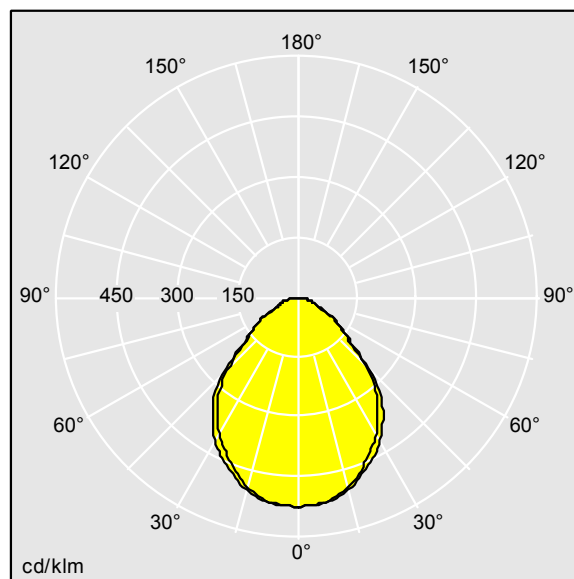
D44261AA_EQL_840_HF_L1000_LRO_WH_.ldt
