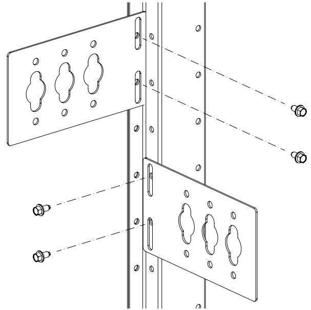
TOP BRACKET ORIENTATION EXAMPE
