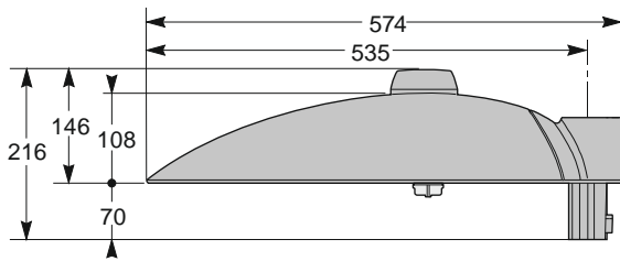
BRP435 Standard Side Entry (Ø 48 mm - Ø 60 mm)
