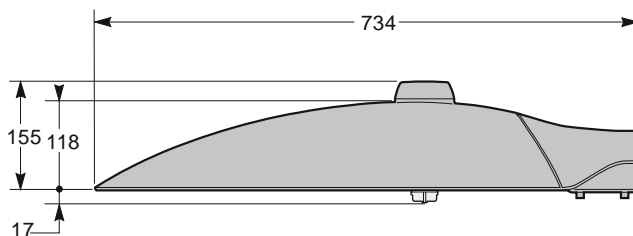
BRP436 Standard Side Entry (Ø 60 mm)
