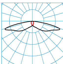
Jovie 50-SB3L-ML/1000-2200-730 2G1 ETDD (CLO initial value) TX271523 ■ C0 - C180 ■ C90 - C270 DIN 5040: A20 UTE: 1,00 l CEN Flux Code: 29 61 91 100 100
