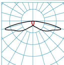
Jovie 50-SB3L-ML/1000-2200-730 2G1 ETDD (1000 lm) TX068693 ■ C0 - C180 ■ C90 - C270 DIN 5040: A20 UTE: 1,00 l CEN Flux Code: 29 61 91 100 100
