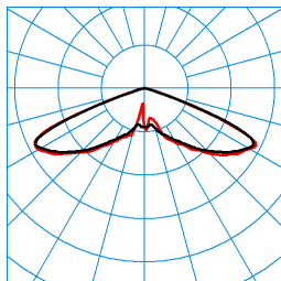
Publisca P1W-RB6L-LRA/2600-730 3G1S ET (CLO end value) TX300967 ■ C0 - C180 ■ C90 - C270 DIN 5040: A20 UTE: 1,00 J CEN Flux Code: 19 57 99 100 100 0 50 50 0
