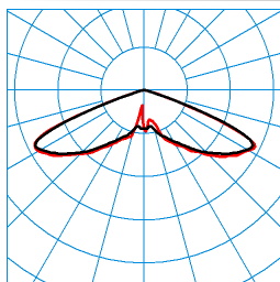
Publisca P1W-RB6L-LRA/2600-730 3G1S TX053547 ■ C0 - C180 ■ C90 - C270 DIN 5040: A20 UTE: 1,00 J CEN Flux Code: 19 57 99 100 100 0 50 50 0
