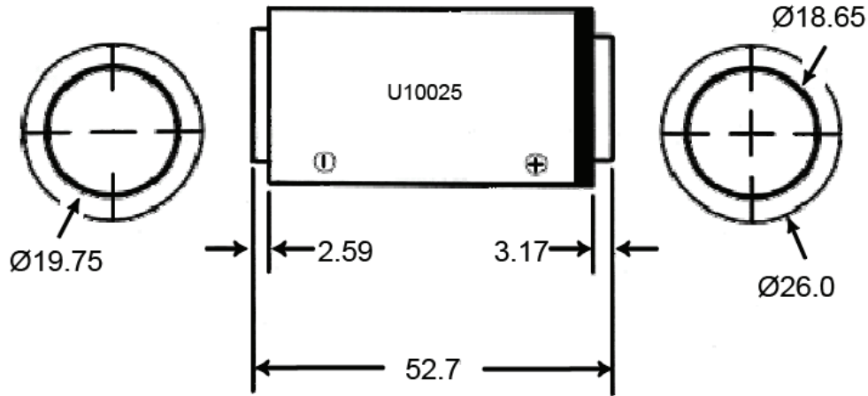
Maximum Dimensions in mm
