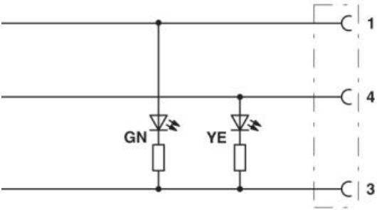
Wiring diagram
