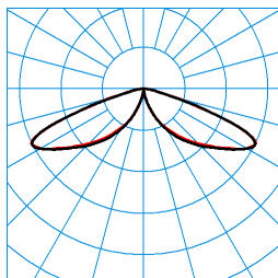
LTX LT-RB6L-LRA/15/18/26-730 4G1 (2600 lm) TX084119 ■ C0 - C180 ■ C90 - C270 DIN 5040: A20 UTE: 1,00 J CEN Flux Code: 15 51 96 100 100 0 0 0 0
