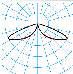
LTX LT-RB6L-LRA/15/18/26-730 4G1 (1500 lm) TX084117 ■ C0 - C180 ■ C90 - C270 DIN 5040: A20 UTE: 1,00 J CEN Flux Code: 15 51 95 100 100 0 0 0 0
