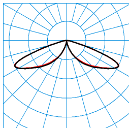
LTX LT-RB6L-LRA/15/18/26-730 4G1 (1800 lm) TX084118 ■ C0 - C180 ■ C90 - C270 DIN 5040: A20 UTE: 1,00 J CEN Flux Code: 15 51 96 100 100 0 0 0 0
