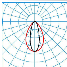
ELINE FL PN60 840 L225 1 20
