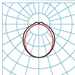
ELINE FL HE+ DL80 865 L225 1 20
