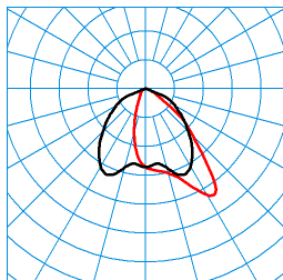
Jovie 70I-AM3L-SLR3/15000-730 12G1 ET (CLO end value) TX300755 ■ C0 - C180 ■ C90 - C270 DIN 5040: A50 UTE: 1,00 D CEN Flux Code: 59 89 100 100 100
