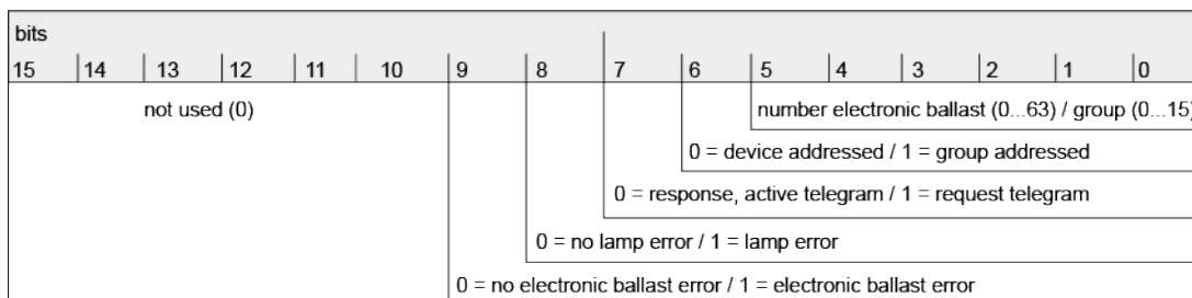
Figure 15: Telegram structure, 2-byte error status
