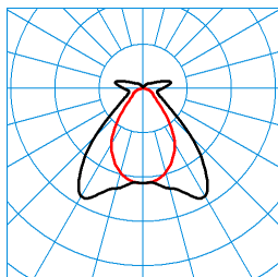
TugraHE Act 15 PW19 50 ETDD 26 (ACTCSU) TX306289 ■ C0 - C180 ■ C90 - C270 DIN 5040: B41 UTE: 0,81 D + 0,19 T CEN Flux Code: 60 85 94 81 100 9 28 64 19
