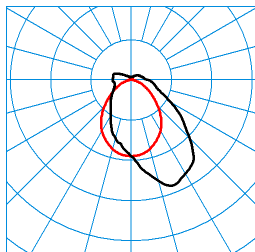
TugraHE 15 PAW 28-89/16ML-830 ET PC 23 (STAG11) TX425207 ■ C0 - C180 ■ C90 - C270 DIN 5040: B40 UTE: 0,86 E + 0,14 T CEN Flux Code: 48 77 92 86 100 13 32 64 14
