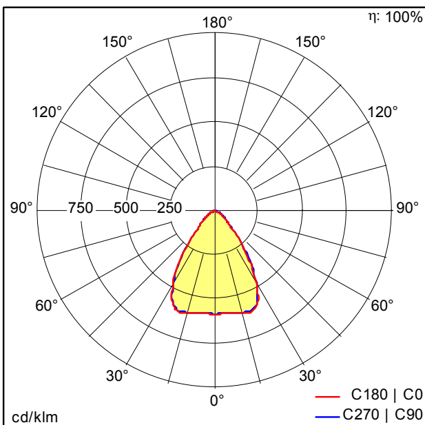
D46450_CR2PL_M13k-840_PM_WB_LDO.ltd
