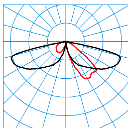
CS 19 100-AB2L/4600-740 4G1S ETDD (CLO initial value) TX300025 ■ C0 - C180 ■ C90 - C270 DIN 5040: A20 UTE: 1,00 l CEN Flux Code: 27 65 96 100 100 0 0 0 0
