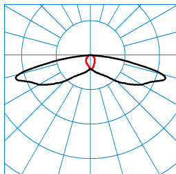
LIQ 50N-SB3L-LR/1650-740 2G1 ET (CLO initial value) TX278019 ■ C0 - C180 ■ C90 - C270 DIN 5040: A30 UTE: 1,00 l CEN Flux Code: 31 64 92 100 100
