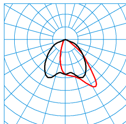
Jovie 70I-AM3L-LRA/18000-740 18G1 ET (CLO initial value) TX301345 ■ C0 - C180 ■ C90 - C270 DIN 5040: A50 UTE: 1,00 D CEN Flux Code: 59 89 100 100 100
