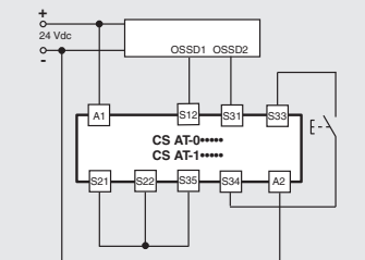
Input configuration with manual start 2 channels
