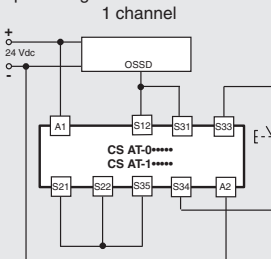
Input configuration with manual start 1 channel
