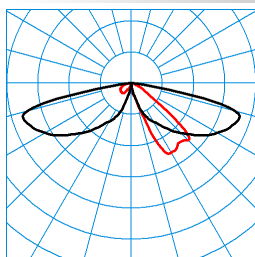
LTX K-AB2L-LRA/15/18/26-740 4G1 (1800 lm) TX062693 ■ C0 - C180 ■ C90 - C270 DIN 5040: A20 UTE: 1,00 l CEN Flux Code: 24 61 92 100 100 0 0 0 0
