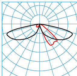
LTX K-AB2L-LRA/15/18/26-740 4G1 (2600 lm) TX062694 ■ C0 - C180 ■ C90 - C270 DIN 5040: A20 UTE: 1,00 l CEN Flux Code: 24 61 92 100 100 0 0 0 0
