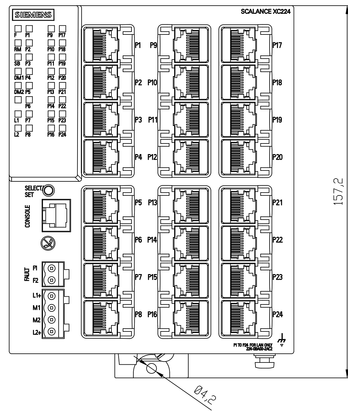
Vorne offen / Front open Alternative Befestigung / Alternative mounting
