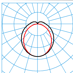
Ridos OT LED3000-830 TX044216
