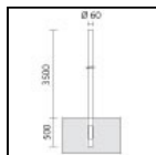
S.2842 POTEAU CYLINDRIQUE H 3,5m  60mm   ENTERRER
