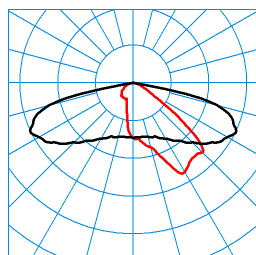
LIQ 50N-AB2L-LR/220/260/320-727 4G1 ET (CLO initial value) TX277999 ■ C0 - C180 ■ C90 - C270 DIN 5040: A30 UTE: 1,00 G CEN Flux Code: 34 71 96 100 100 0 0 0 0
