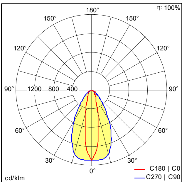
D44423AA_TEC_LED10000-865_L2000_NB_LDE_WH_IP.ltd
