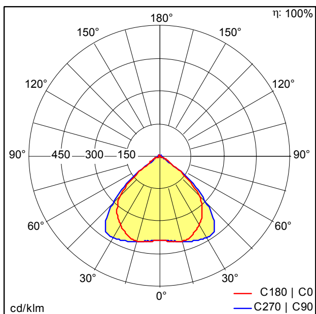
KXA-2_52W_LED_840.ltd
