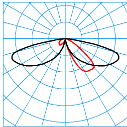
LTX PT-AB2L-LRA/15/18/26-740 4G1 (1800 lm) TX084151 ■ CO - C180 ■ C90 - C270 DIN 5040: A20 UTE: 1,00 l CEN Flux Code: 23 60 91 100 100 0 0 0 0
