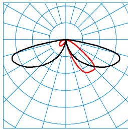
LTX PT-AB2L-LRA/15/18/26-740 4G1 (2600 lm) TX084152 ■ CO - C180 ■ C90 - C270 DIN 5040: A20 UTE: 1,00 l CEN Flux Code: 23 60 91 100 100 0 0 0 0
