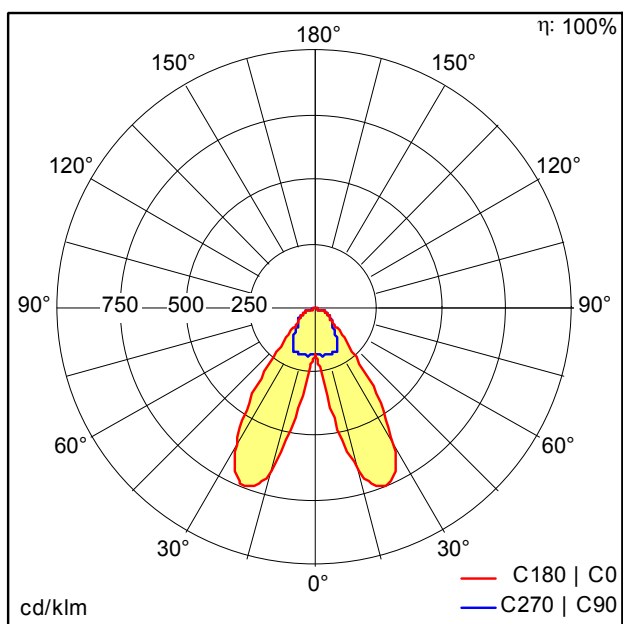
D43655AA_TECTON_C_LED5500-865_L1500_SB_EVG_WH.Idt
