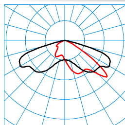
LIQ 90-AB7L-SLR2/29000-740 24G1S TX122197 ■ C0 - C180 ■ C90 - C270 DIN 5040: A30 UTE: 1,00 l CEN Flux Code: 33 72 98 100 100
