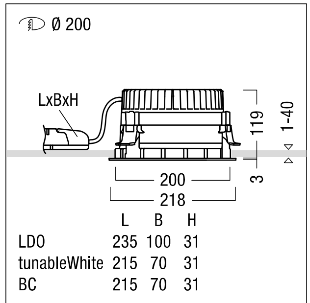
ZS_PA1_M_R200H_LED_WH.wmf
