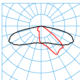
LIQ 50N-AB2L-LRA/2400-740 4G1 ETDD (CLO initial value) TX278208
