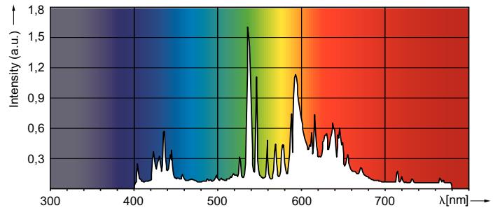
Spectral Power Distribution Colour - MASTERC CDM-T 250W/830 G12 1CT/12
