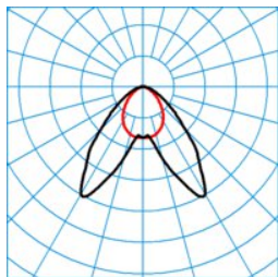
ELINE LDAW55-140 ML 865 L225 4 20 ■ C0 - C180
