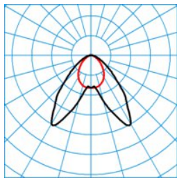
ELINE LDAW55-140 ML 865 L225 2 20 ■ C0 - C180
