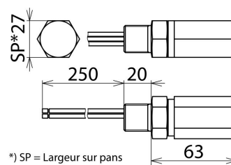
Dimensions CD EXI+D 2X24 M
