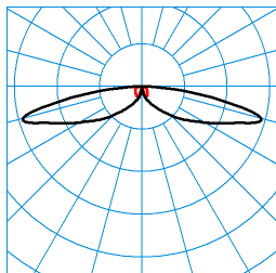
CS 19 100-SB3L-SLR1/2200-730 2G1S ET (CLO initial value) TX300156 ■ C0 - C180 ■ C90 - C270 DIN 5040: A20 UTE: 1,00 J CEN Flux Code: 22 52 84 100 100 0 0 0 0
