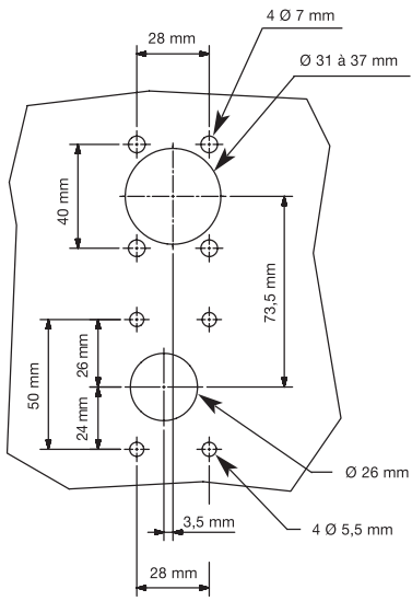
S1 - S2 - S3 type Type S1 - S2 - S3
