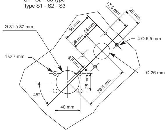
S4 type Type S4
